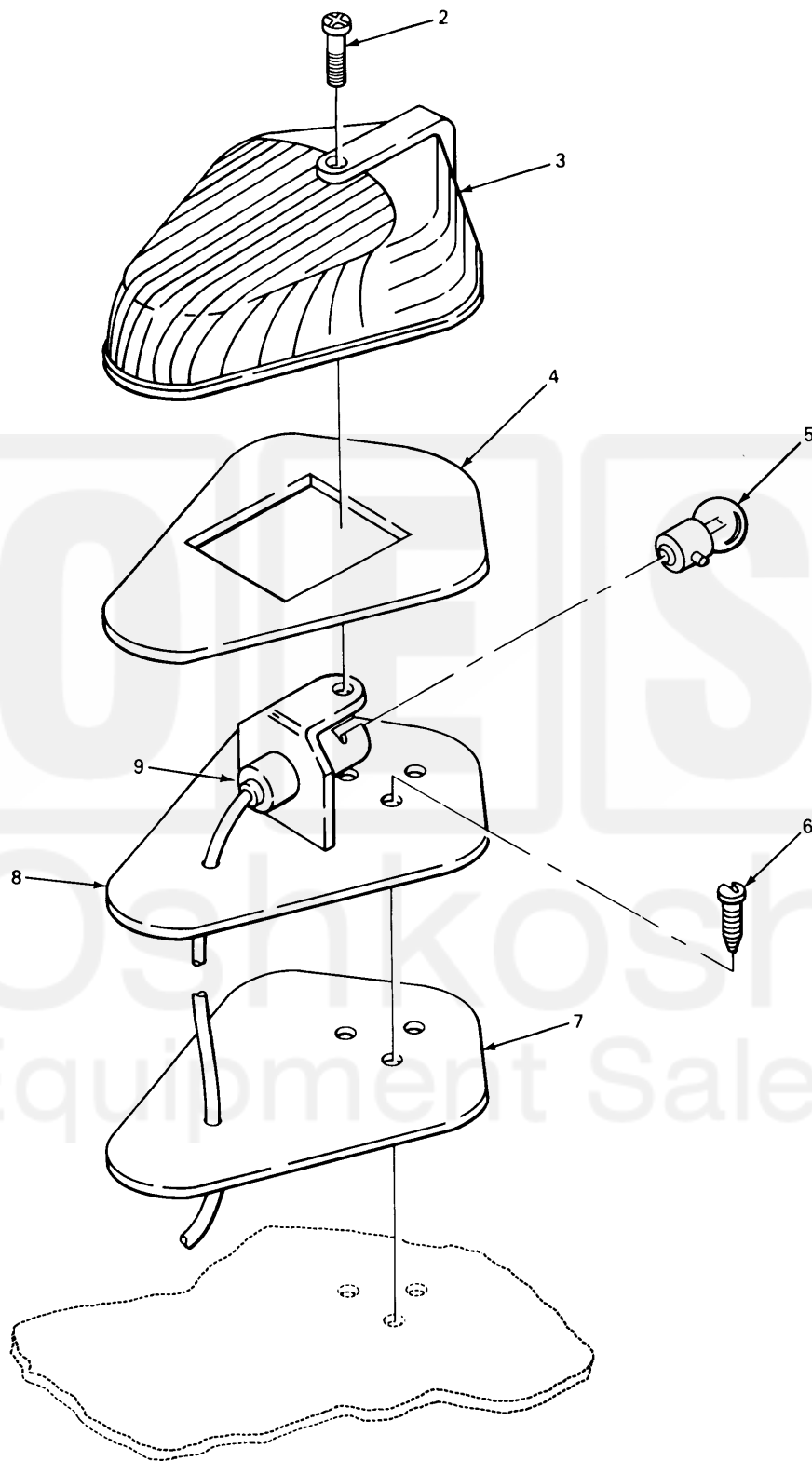
FIGURE 84. CLEARANCE LIGHT.
